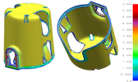
Design for Manufacturing (DFM) Analysis
